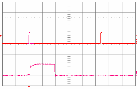
Fig. 27: Load current (top trace, 20 A/div, 20 ms/div) into a 10 mΩ short circuit during restart, at V in = 24 V. Bottom trace (20 A/div, 1 ms/div) is an expansion of the on-time portion of the top trace.
